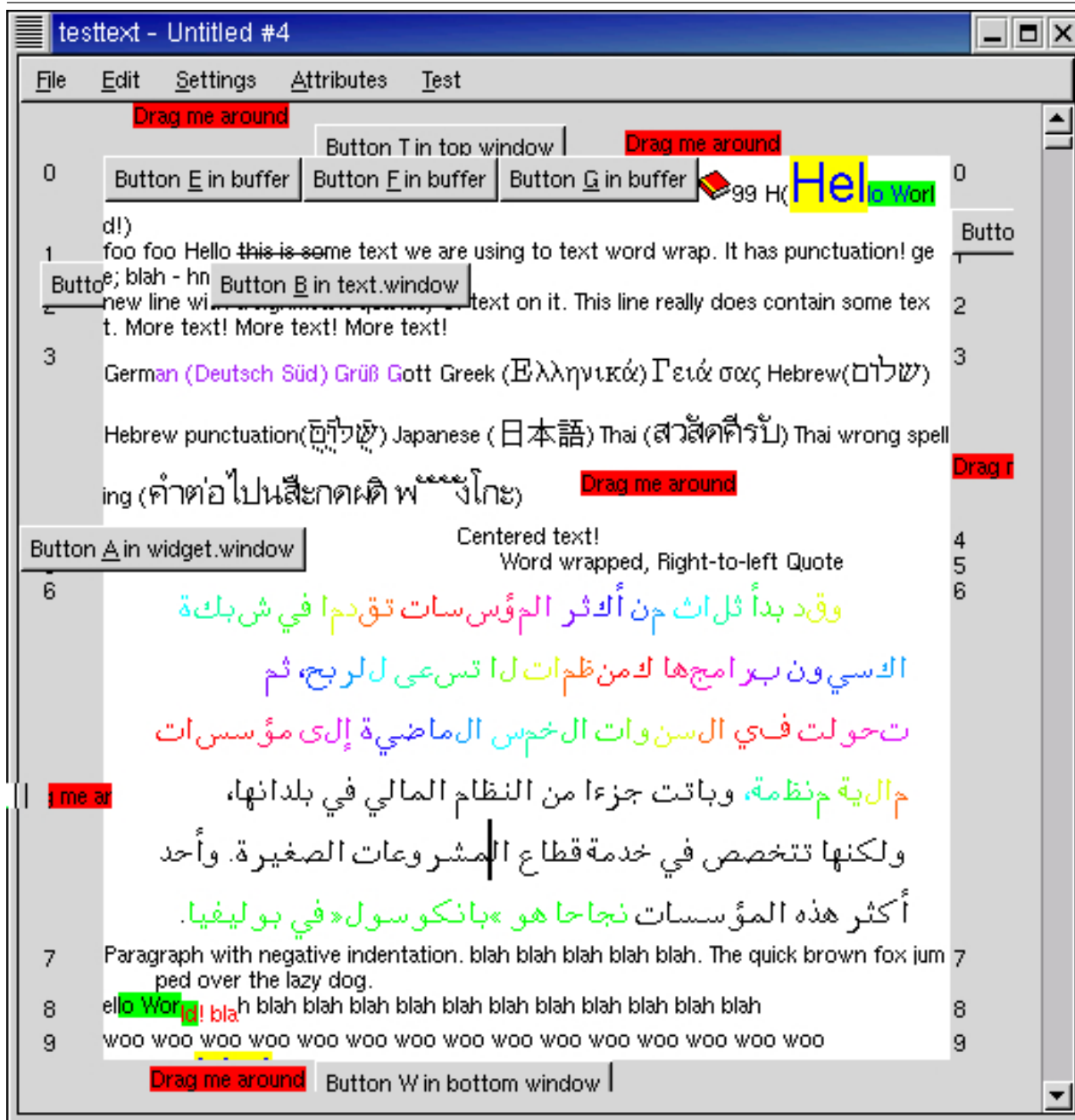
Figure 13.2 TextView Example
